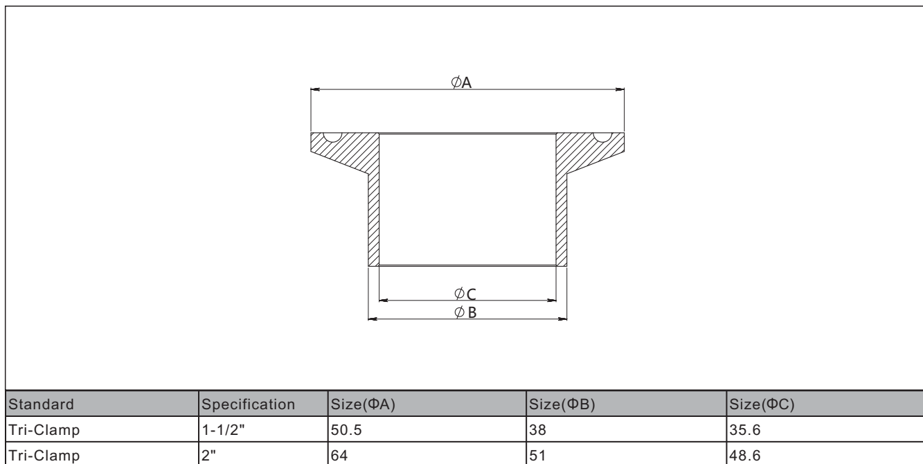
Welding adapter(Z1-Z2) (unit: mm )
