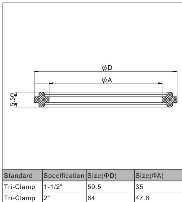
Sealing gasket(M1-M2)(unit: mm)
