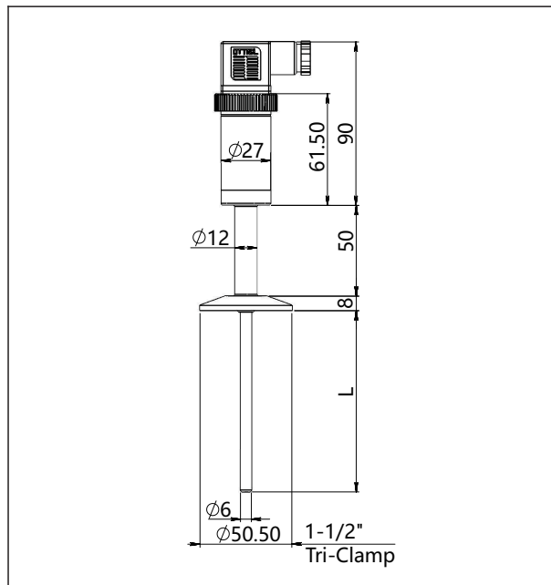
Process connection(G01) (unit: mm)
