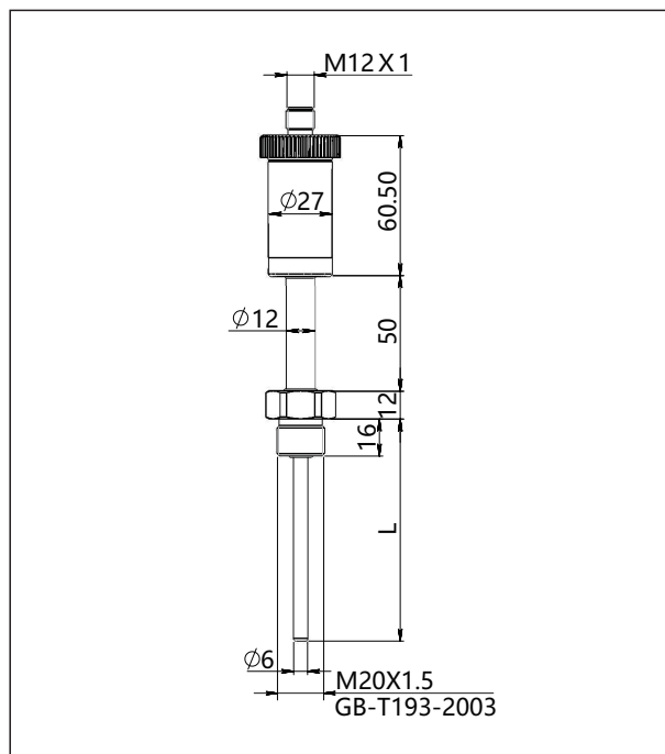
Drawing and dimension (thread) with aviation plug (H1) and extension tube(unit: mm)
